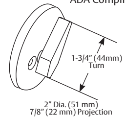
Inside Turn Lever ADA Compliant
